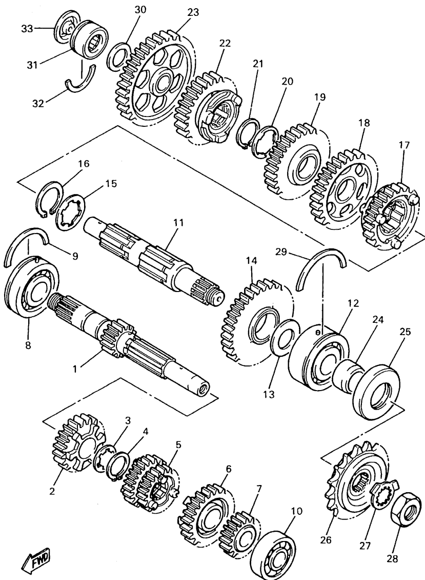
FIG. 17 TRANSMISION
