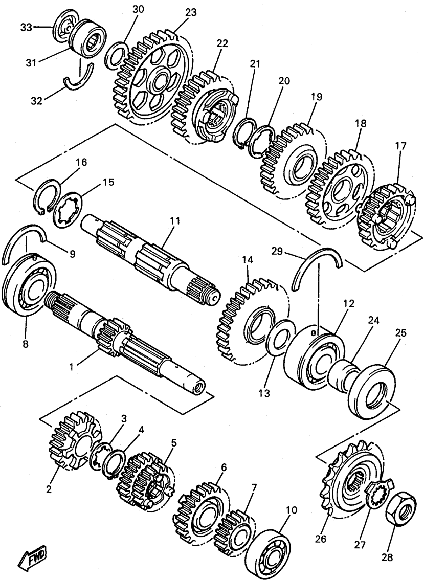
FIG. 17 TRANSMISION
