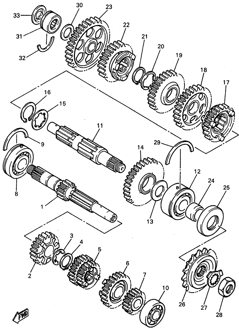
FIG. 17 TRANSMISION
