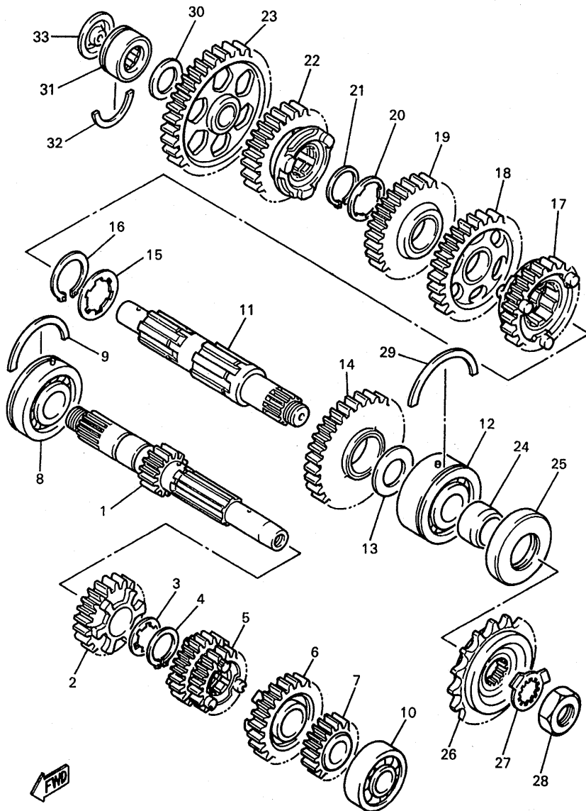
FIG. 17 TRANSMISION
